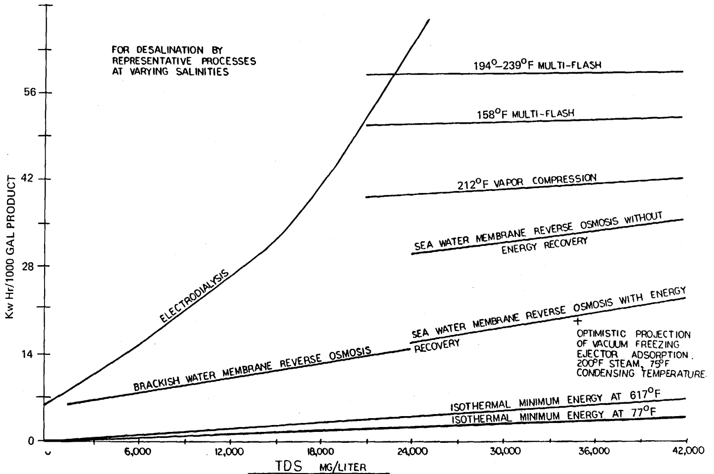
Figure 4-1. Energy consumption.
